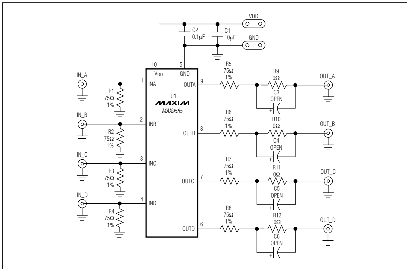
Figure 1. MAX9585 EV Kit Schematic
